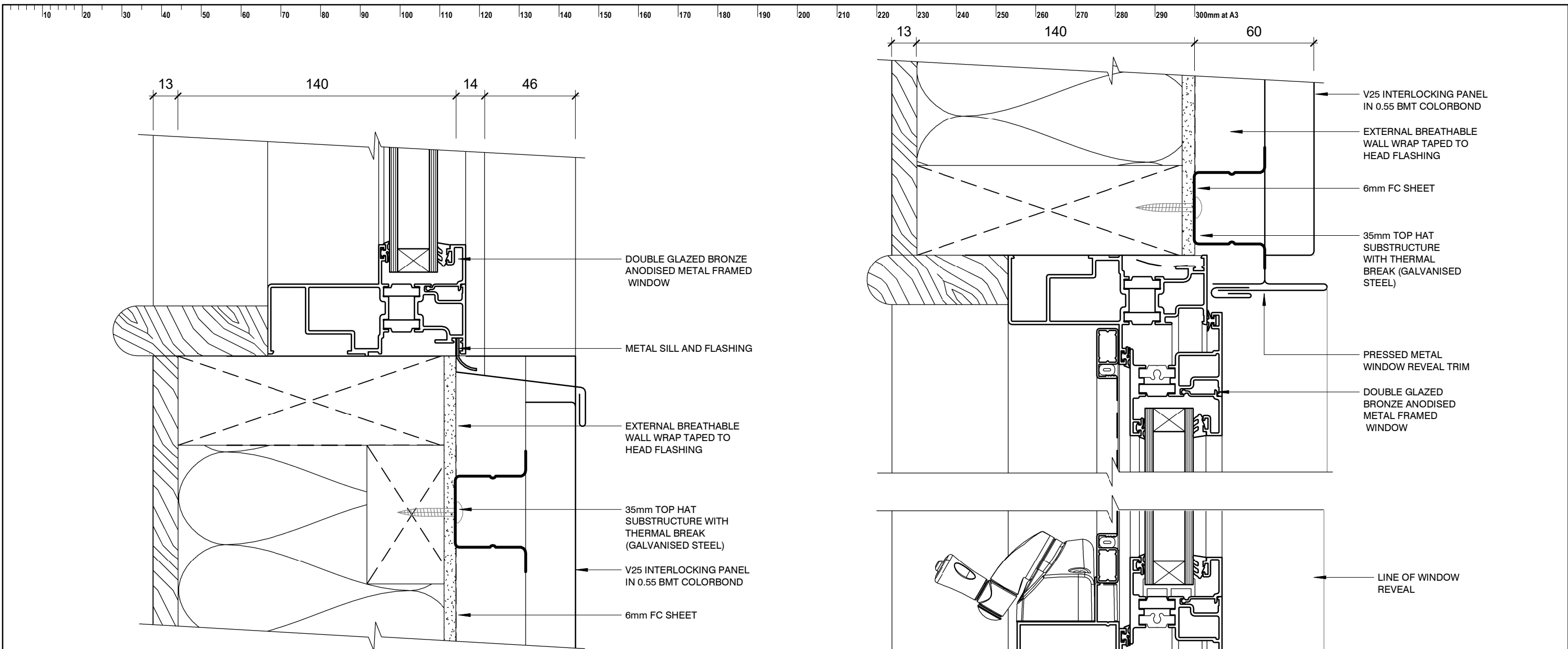
01 D01 HORIZONTAL SECTION - FIXED DOUBLE GLAZED WINDOW DETAIL 1 : 2
